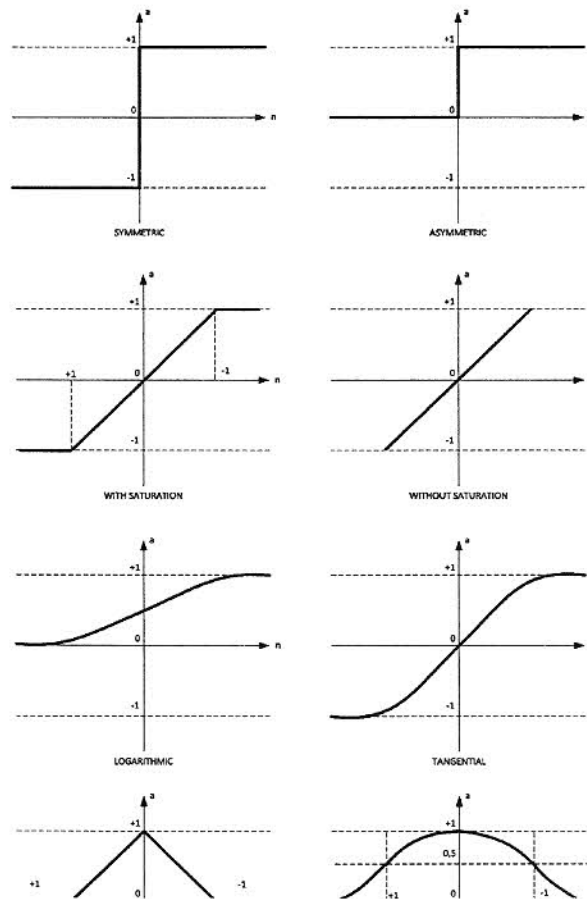
Figure 12: Example of different kind of transfer functions.
