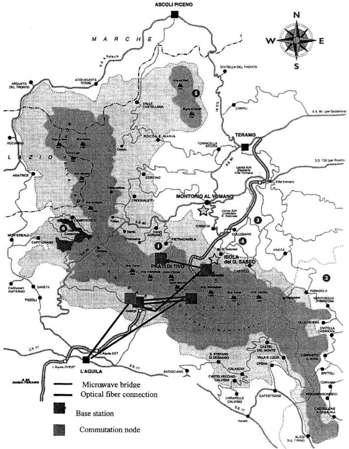
Figure 10: Positioning of the communication devices outside the Gran Sasso Mountain.
