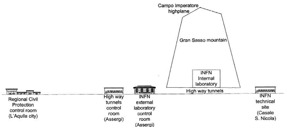
Figure 4: Transversal schematization of Gran Sasso Mountain system.
