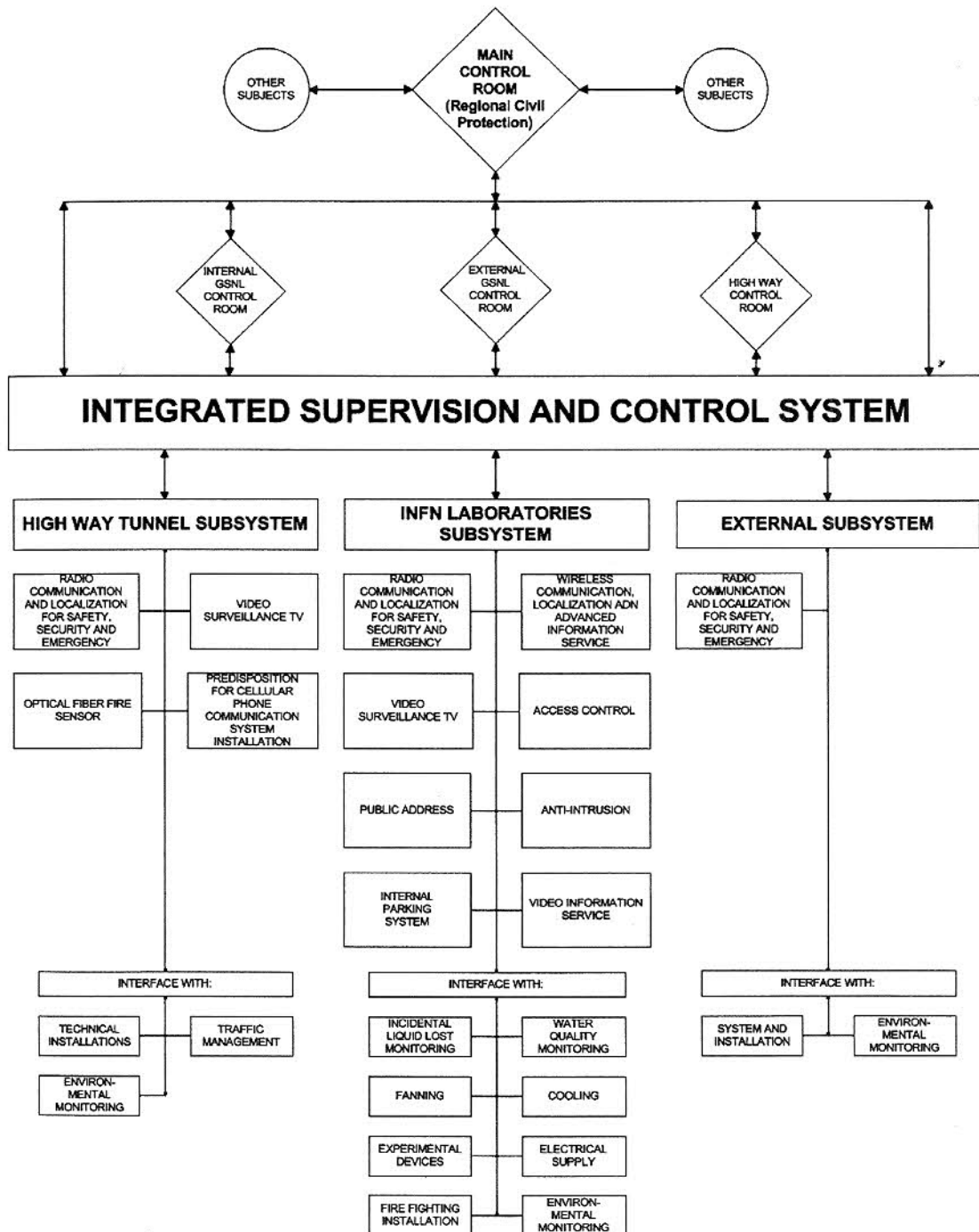
Figure 5: Functional blocks diagram of the integrated system.
