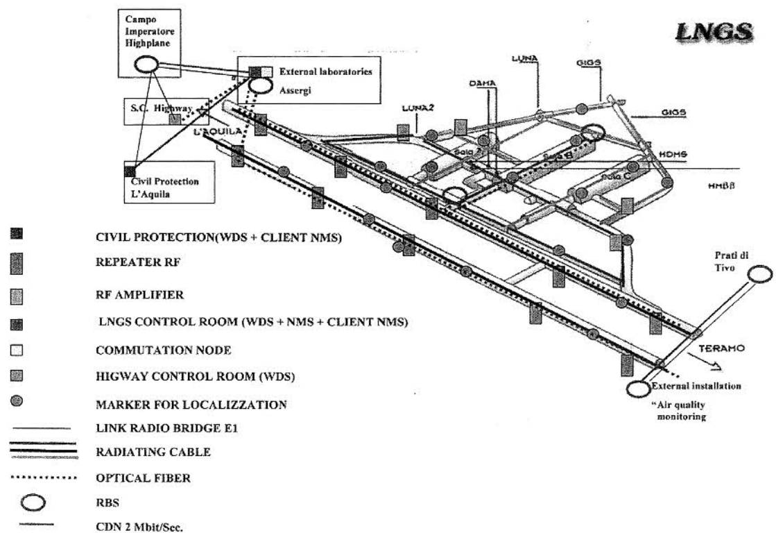
Figure 8: Scheme of the internal radio communication subsystem.
