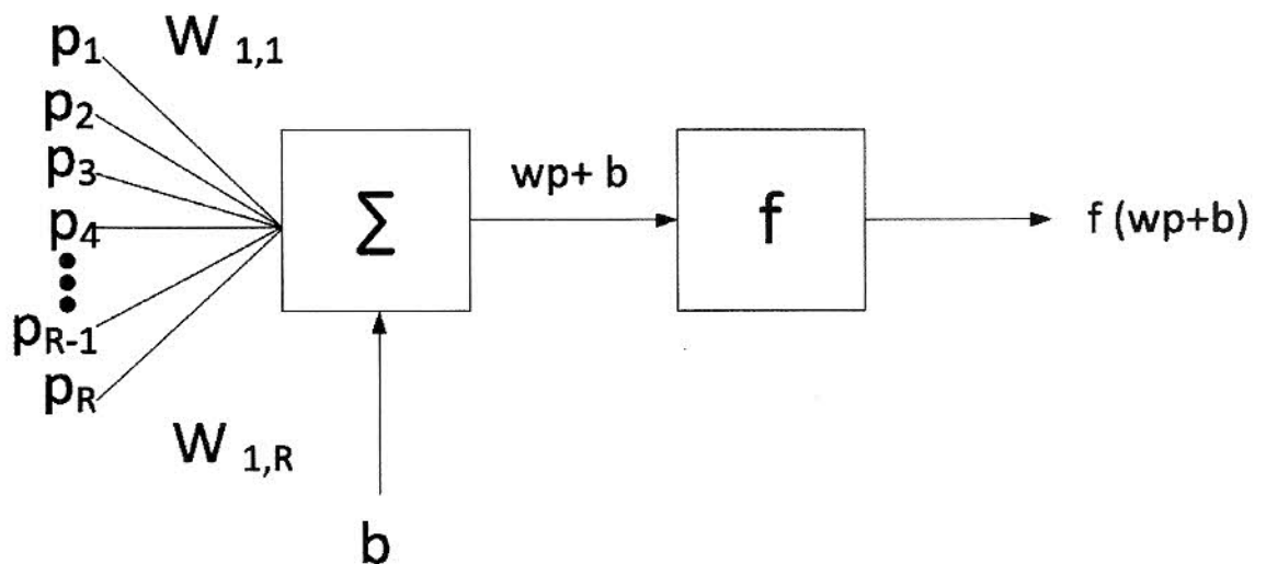
Figure 13: Multiple input neuron.
